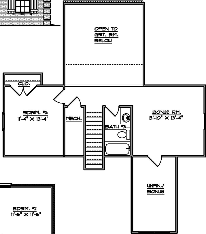
SECOND FLOOR PLAN SCALE: NONE
