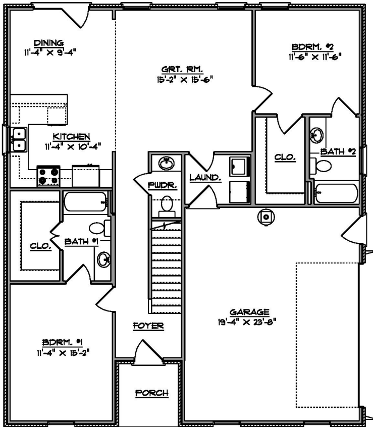
FIRST FLOOR PLAN SCALE: NONE
